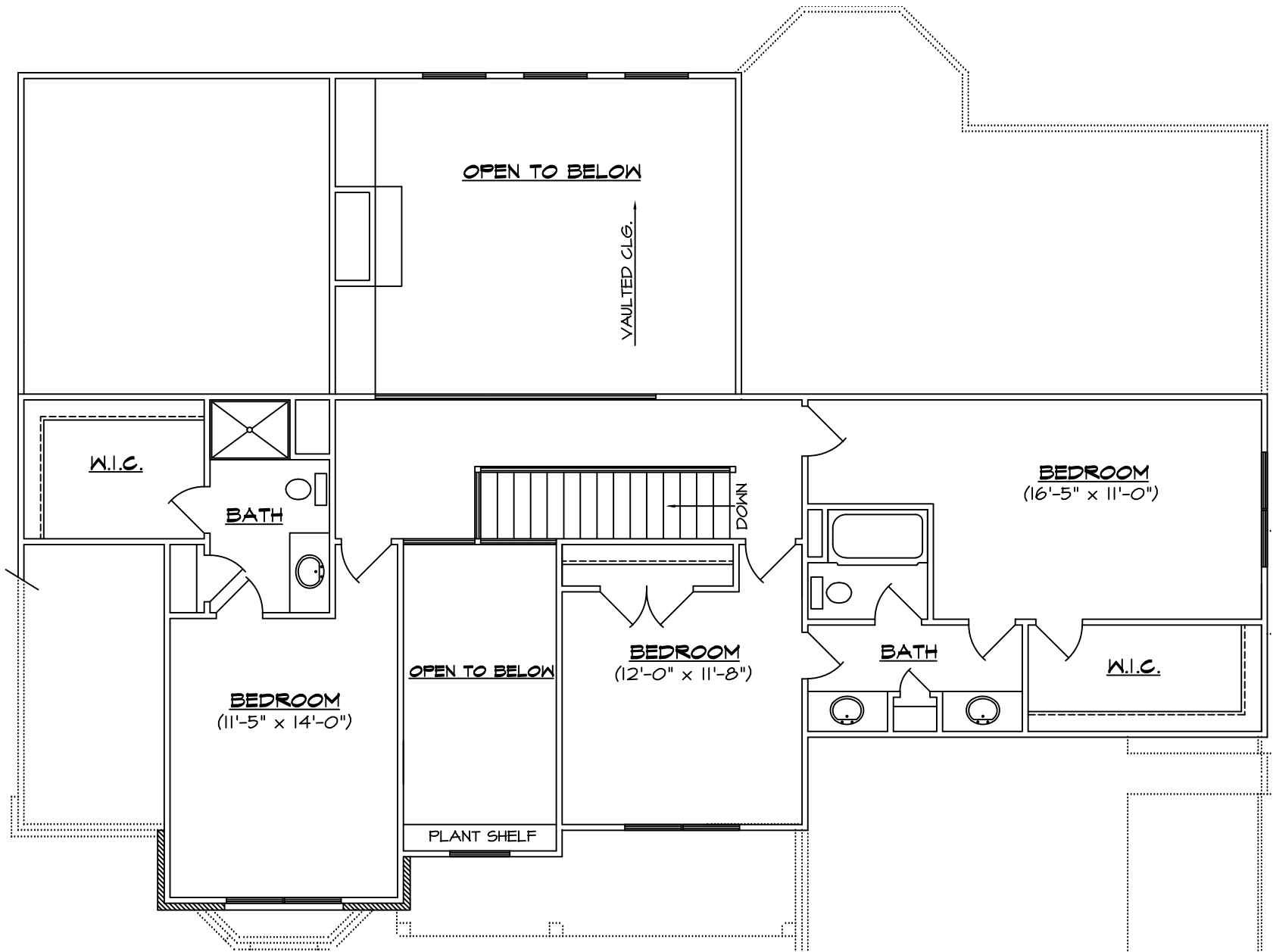
SECOND FLOOR PLAN 1112 SQ. FT.
