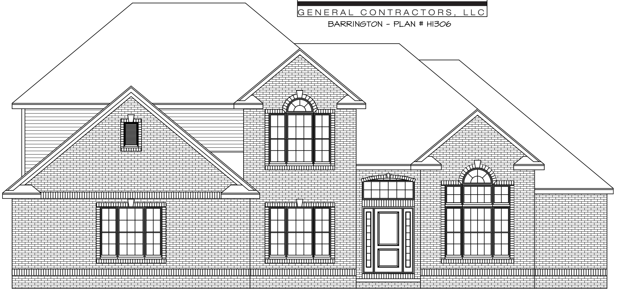
FRONT ELEVATION
